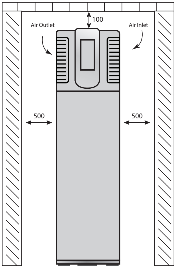
Diagram 2b. Front View 180L
