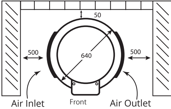
Diagram 1a. Top View 270L
